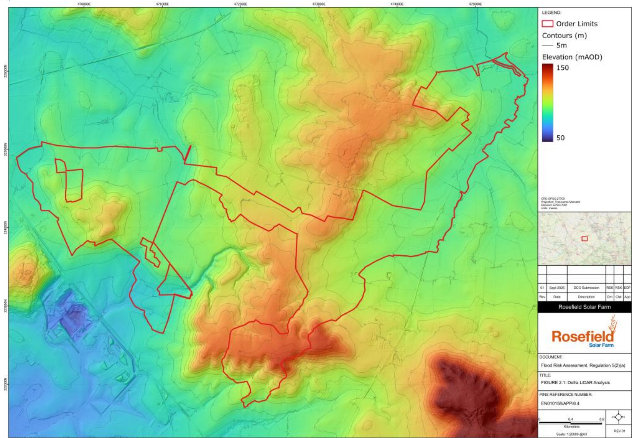
Figure 2.1 : QGIS LiDAR Analysis (Defra)
