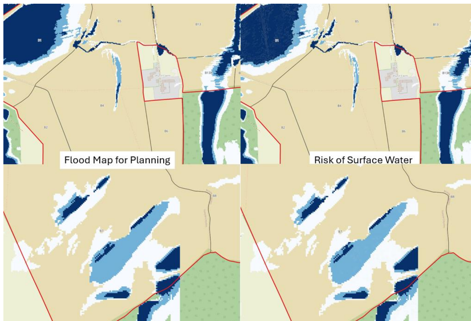
Figure 3.15: Environment Agency RoFSW vs FMFP Surface Water Extents Difference
