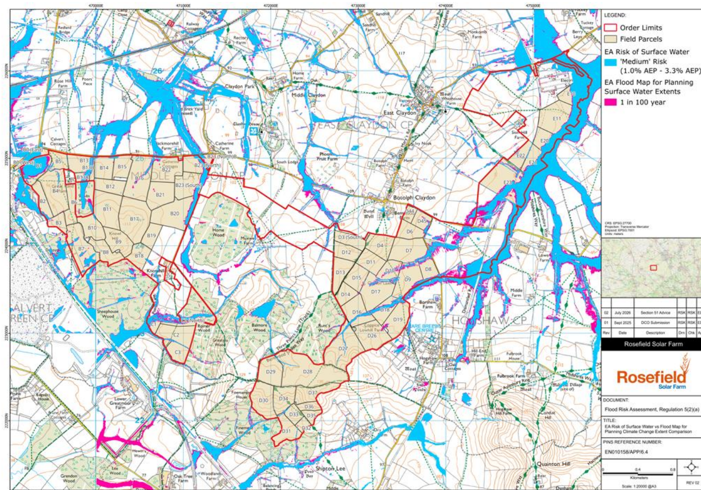
Figure 3.16: Environment Agency Risk of Surface Water ('Medium Risk') vs Flood Map for Planning (1 in 100 year) Climate Change Extents Comparison
