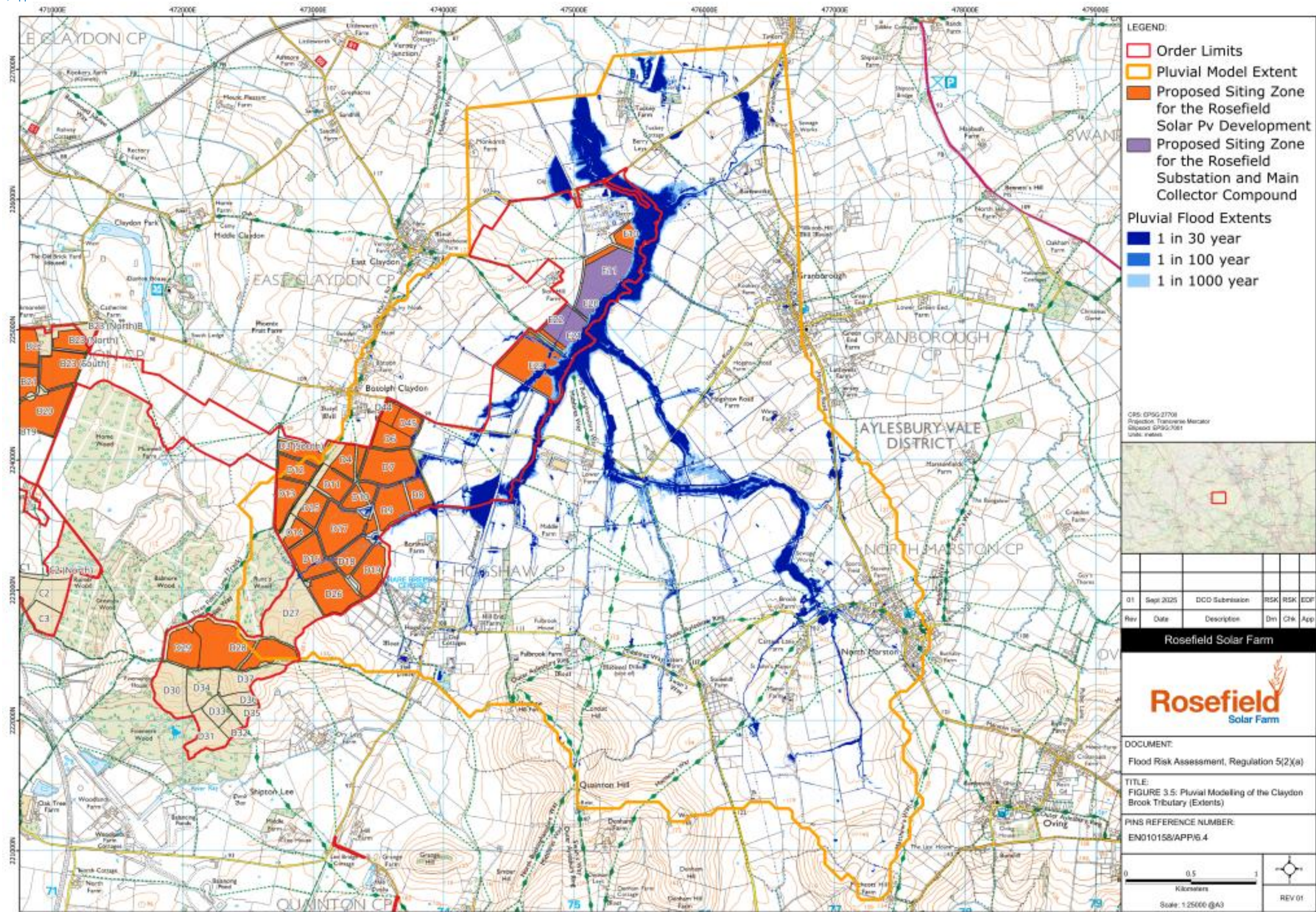
Figure 3.12: Pluvial Modelling of Claydon Brook Tributary
