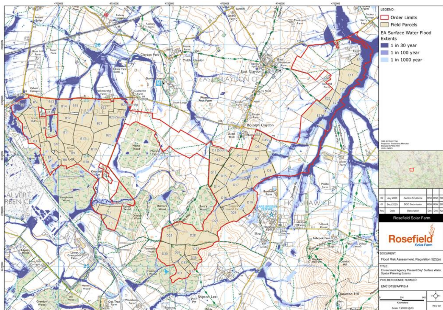
Figure 3.14: Environment Agency Flood Map for Planning 'Present Day' Surface Water Spatial Planning Extents
