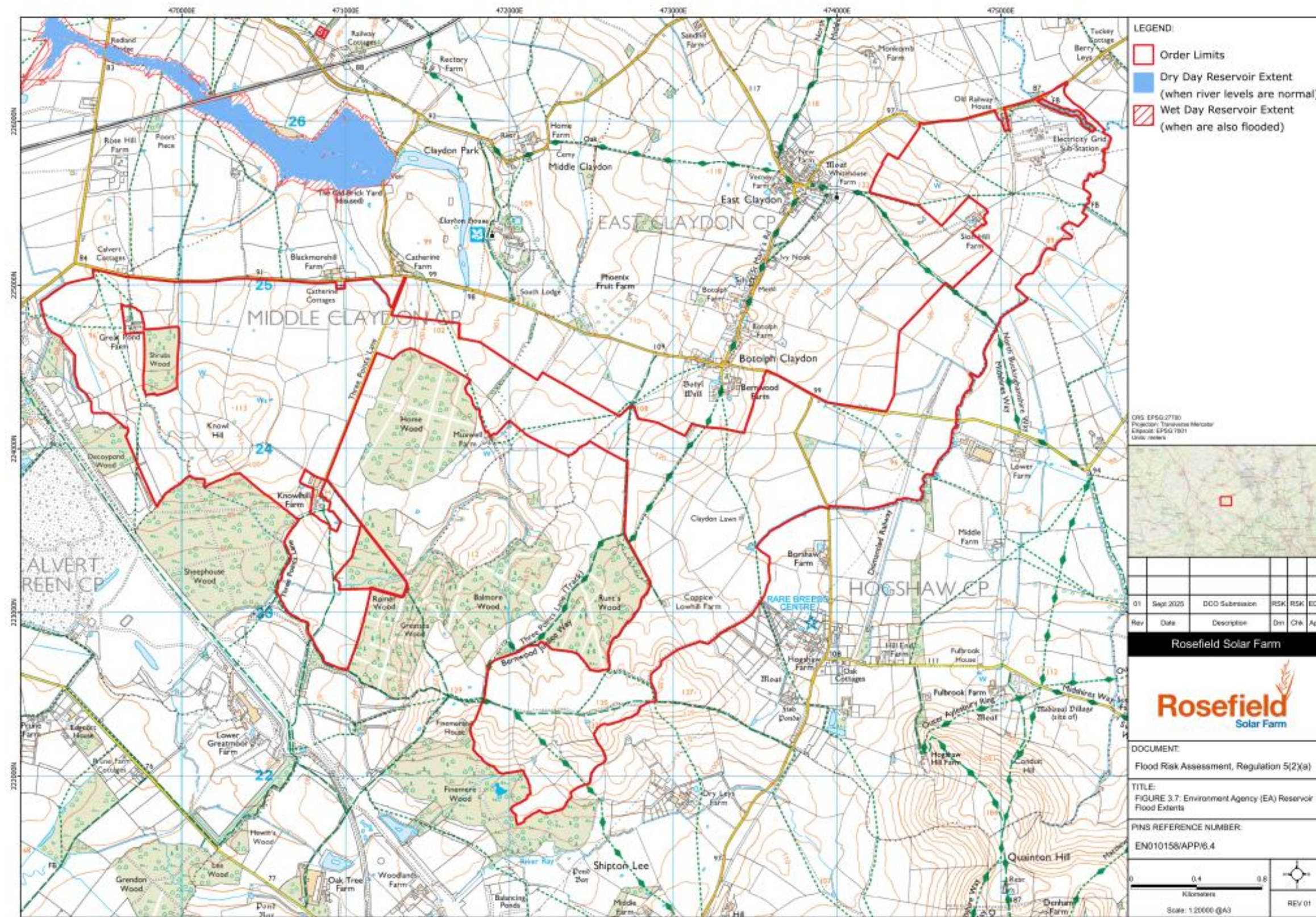
Figure 3.18: Environment Agency Reservoir Flood Extents
