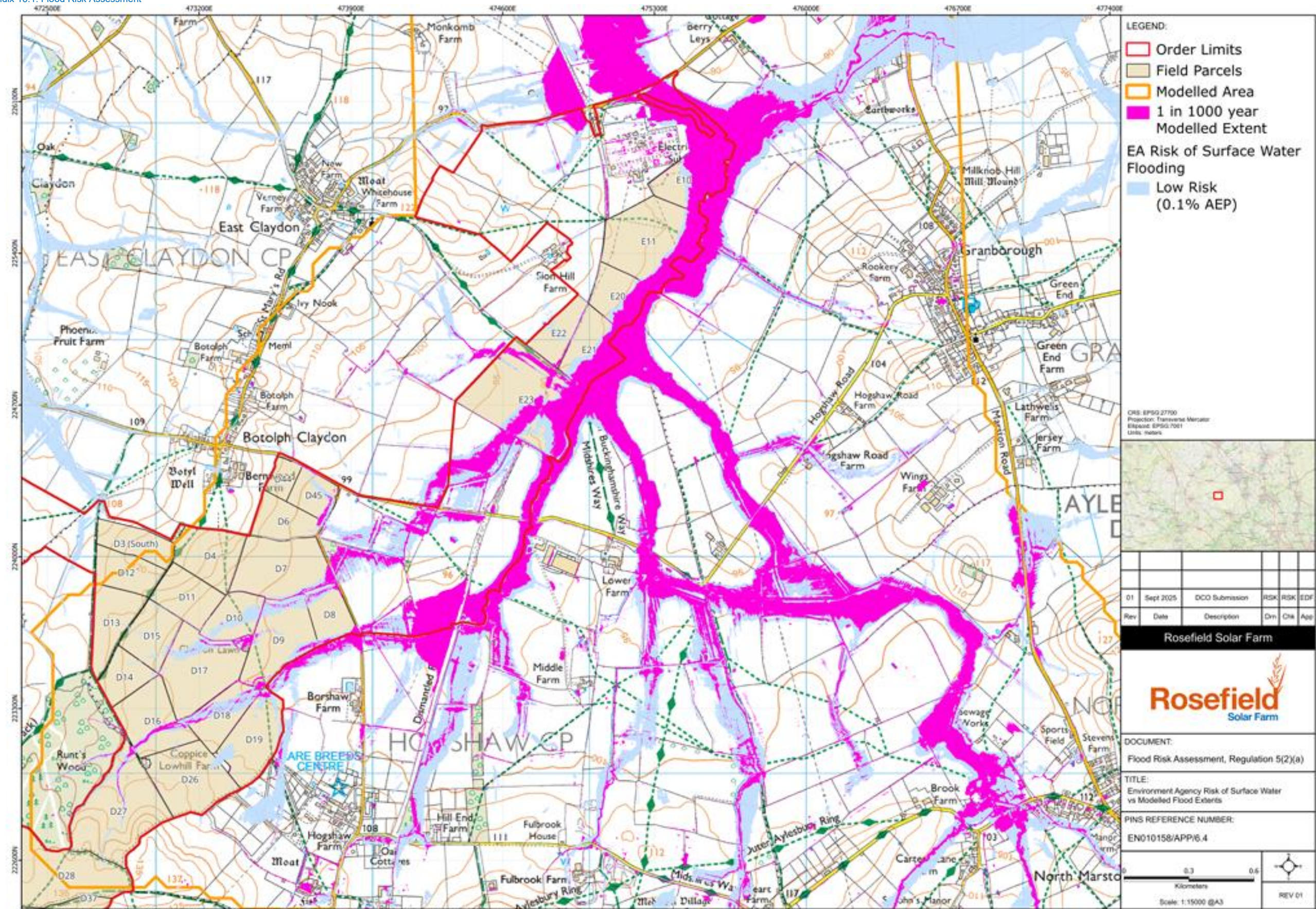
Figure 3.7: Environment Agency 'Low' Risk of Surface Water and Modelled Q1000 Pluvial Extent Comparison
