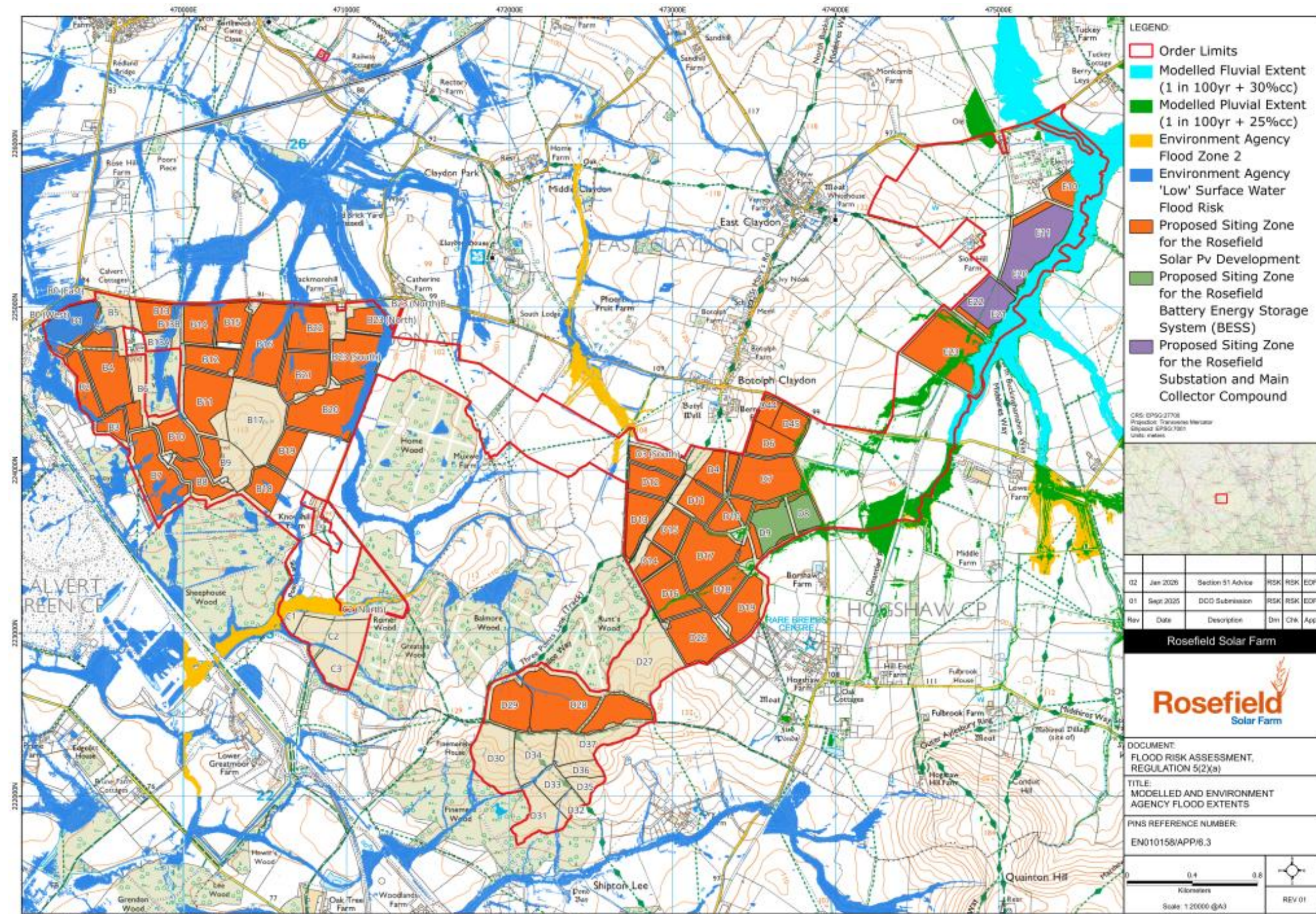
Figure 3.10: Credible Maximum Flood Extents
